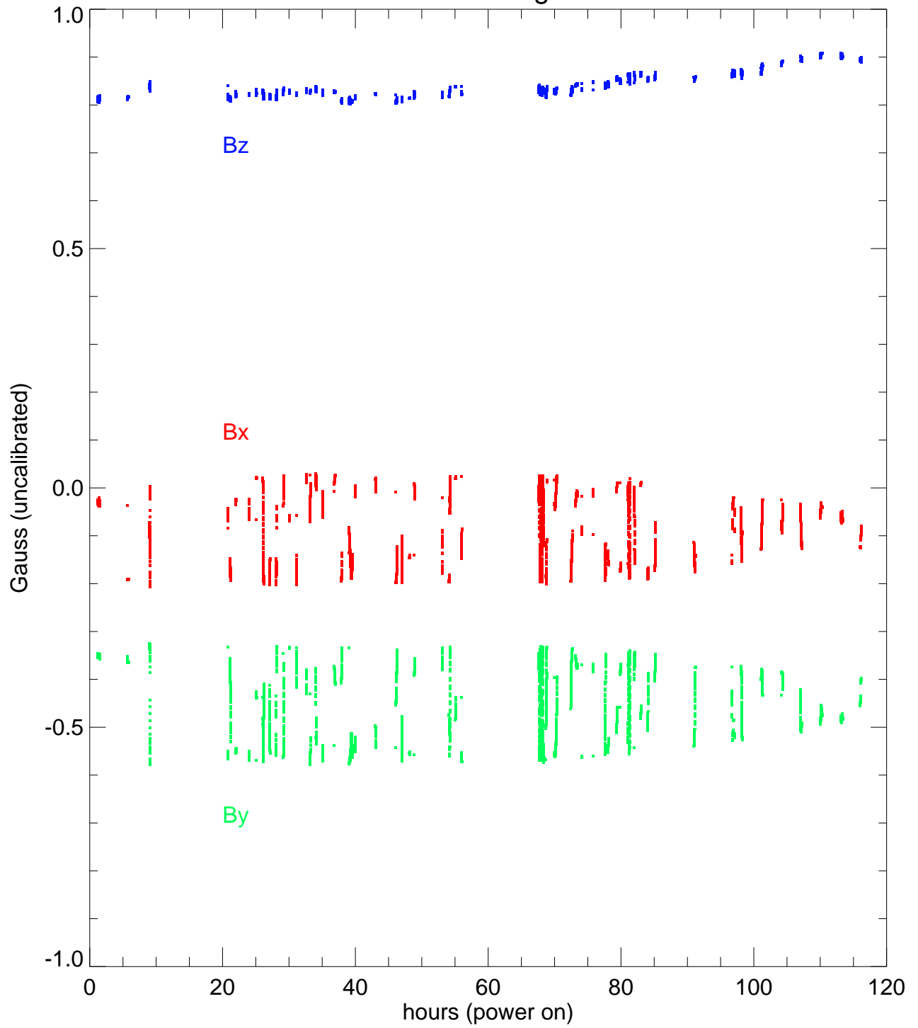
Sweden Jun06 magnetometer
