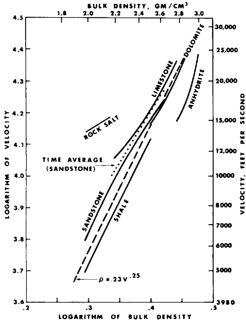
FIG. 1. Velocity-density relationships in rocks of different lithology.
