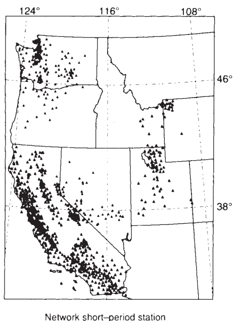
FIG. 1 Location of the 881 stations in the five regional short-period arrays assembled in this study.
