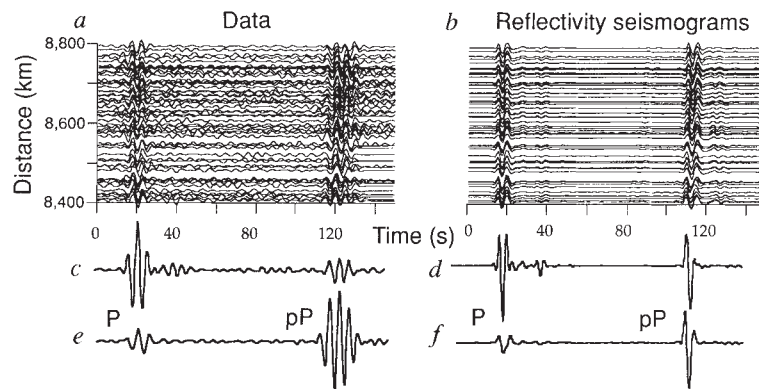
FIG. 3 a, Seismograms from 70 of the 279 stations used to study the 3 April 1985 earthquake, which cover only a quarter of the aperture of our array. All seismograms are aligned on the pP phase. b, Reflectivity seismograms for the same 70 stations. The IASP91 velocity model is used 31 , and the centroid moment tensor mechanism 32 is assumed. The synthetics are filtered in the same way as the data. c, d, Stacks of the data and reflectivity seismograms with the P arrivals aligned. e, f, Stacks of the data and reflectivity seismograms with the pP arrivals aligned.
