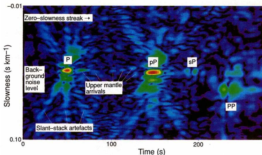
FIG. 4 Slant stack of 3 April 1985 Bonin earthquake. Seismograms from 279 stations are aligned on the P wave and slant-stacked in the time window between P and pP. The logarithms of the envelopes of the stacks are shown. 'Hotter' colour indicates more energy in the stack, with red representing 100 times larger amplitude than black. For example, pP arrives \sim 100 s after P and differs in slowness across the array by 0.003 \text{ s km}^{-1} . This difference in slowness corresponds to a difference in angle of incidence of \sim 1^\circ , or a difference of 5 s between the pP–P times at the opposite ends of the array.
