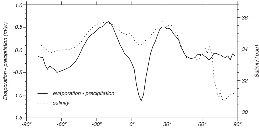
Figure 6.5 Zonal average of sea-surface salinity calculated for all ocean from Levitus (1982) and the difference between evaporation and precipitation ( E - P ) calculated from data shown in figure 5.12.
