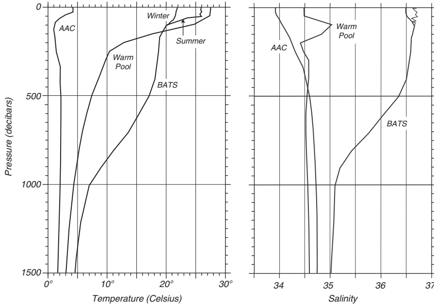
Figure 6.8 Typical temperature and salinity profiles in the open ocean. AAC: At 62.0^\circ S, 170.0^\circ E in the Antarctic Circumpolar Current on 16 January 1969 as measured by the R/V Hakuho Maru . Warm Pool: At 9.5^\circ N 176.3^\circ E in the tropical west Pacific warm pool on 12 March 1989 as measured by Bryden and Hall on the R/V Moana Wave . BATS: At 31.8^\circ N 64.1^\circ W near Bermuda on 17 April and 10 September 1990 as measured by the Bermuda Biological Station for Research, Inc. Data are included with Java OceanAtlas.
