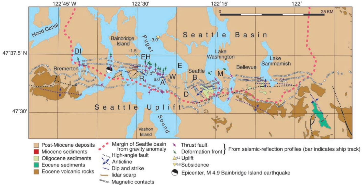
Figure 3. Geologic compilation of the area including the Seattle fault zone and Seattle uplift, simplified from Yount and Gower (1991), Frizzell et al. (1984), and Tabor et al. (1993). Seismic-reflection interpretation from Johnson et al. (1999). Uplift data from Atwater and Moore (1992) and R.C. Bucknam (2001, written commun.); values reported as elevation of pre-uplift (or pre-subsidence) shoreline relative to present mean highest high water (MHHW). White dots indicate magnetic contacts interpreted from aeromagnetic data and discussed in text. A—Alki Point, D—Duwamish River, B—Beacon Hill, W—West Seattle, M—Mercer Island, E—Elliott Bay, R—Restoration Point, EH—Eagle Harbor, DI—Dyes Inlet.
