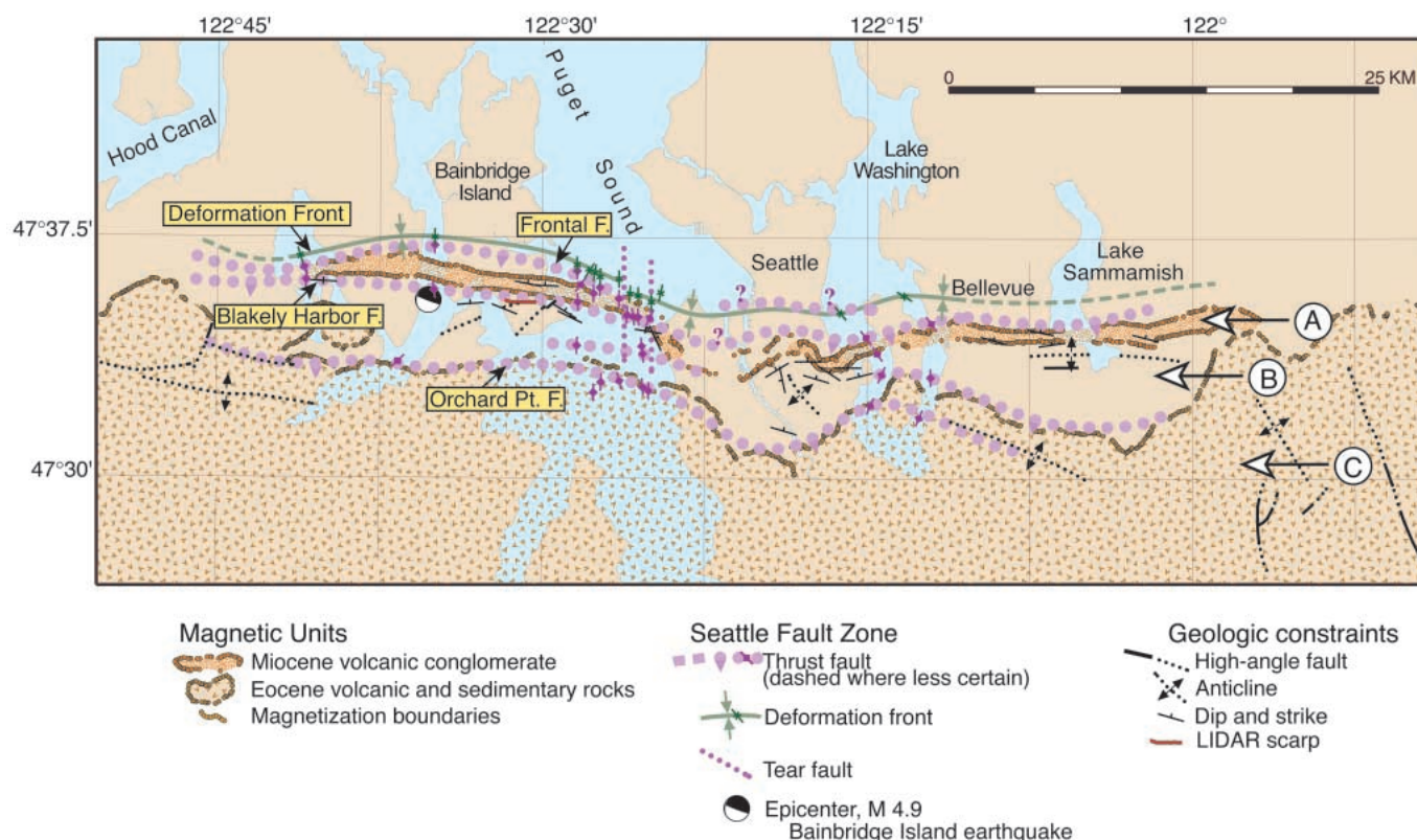
Figure 4. Interpretation of aeromagnetic, generalized geology, and seismic-reflection data of the area including the Seattle fault zone and Seattle uplift. Stipple patterns show interpreted magnetic terranes. Faults are indicated by purple lines, and the deformation front by a green line. Letters A, B, and C indicate anomalies discussed in text.
