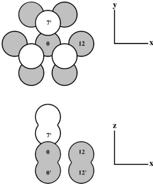
Figure 14 The crystal structure of \beta -oxygen viewed along and normal to the threefold axis. ( Unshaded circles, upper panel ) Above the plane of the shaded atoms.
