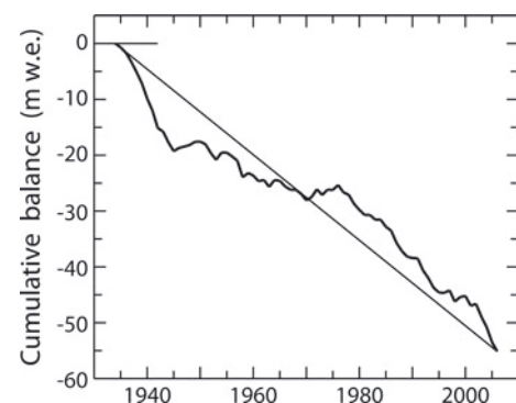
Fig. 7. Cumulative reconstructed–observed B_n from 1935, adjusted to 1970 topography.
