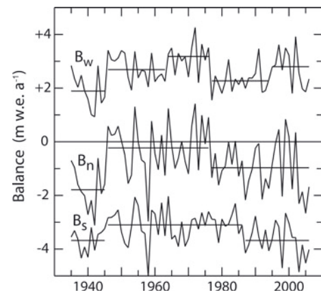
Fig. 6. Reconstructed and observed mass-balance components referring to 1970 glacier topography. For five of the seven shifts P(t) < 0.005 ; for 1963/64 for B_w it is \sim 0.05 and for 1994/95 for B_w it is \sim 0.02 . See Table 3 for dates of stages.
