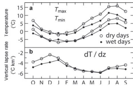
Fig. 4. Mean 1993–2005 climatological conditions at 1848 m, adjacent to South Cascade Glacier: (a) mean daily maximum temperature T_{\max} (upper curve) and minimum temperature T_{\min} (lower curve) on days with Diablo Dam precipitation P > 1 mm (closed circles) and P \leq 1 mm (open circles); and (b) vertical lapse rate of mean temperature between 1848 m and Diablo Dam (271 m).
