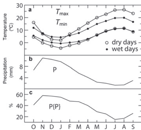
Fig. 2. Mean 1945–2006 climatological conditions at Diablo Dam: (a) mean daily maximum temperature T_{max} (upper curve) and minimum temperature T_{min} (lower curve) on days with precipitation P > 1 mm (closed circles) and with P \leq 1 (open circles); (b) mean daily P in mm\ d^{-1} ; and (c) fraction of days with P > 1 .
