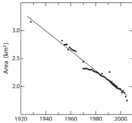
Fig. 3. Decreasing glacier area with unweighted best-fitting straight line. Data from 15 sources.
