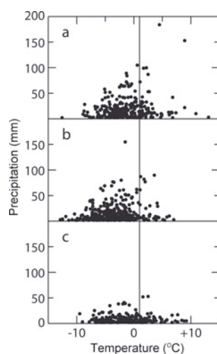
Fig. 5. Joint distribution of precipitation P at Diablo Dam (mm) and temperature T at 1848 m adjacent to South Cascade Glacier during balance years 1998–2005 for (a) autumn (mid-October to mid-December, 247 days, snow fraction 70%); (b) winter (mid-December to mid-March, 340 days, snow fraction 87%); and (c) spring (mid-March to mid-May, 197 days, snow fraction 75%). The rain–snow divide is indicated by the vertical line at T = +1^\circ\text{C} .
