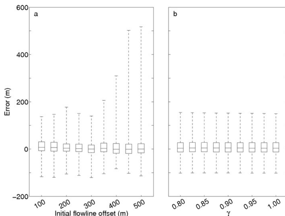
Fig. 4. Results of analysis of calculated ice thickness sensitivity to changes in (a) initial flowline offset, and (b) \gamma (Eqns (3–6)). Error is defined as the difference between measured and calculated ice thicknesses.
