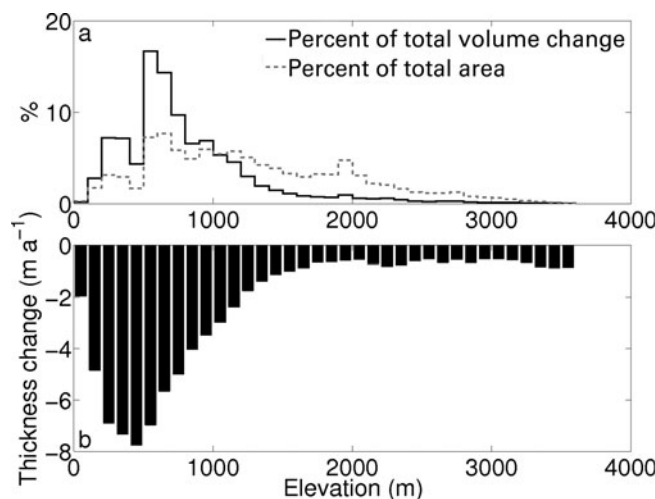
Fig. 9. (a) Percent of total volume change 1957–2007, along with percent of total area (1957 hypsometry), and (b) thickness change 1957–2007 for each 100 m elevation band (from 0 to 3700 m; 1957 hypsometry).
