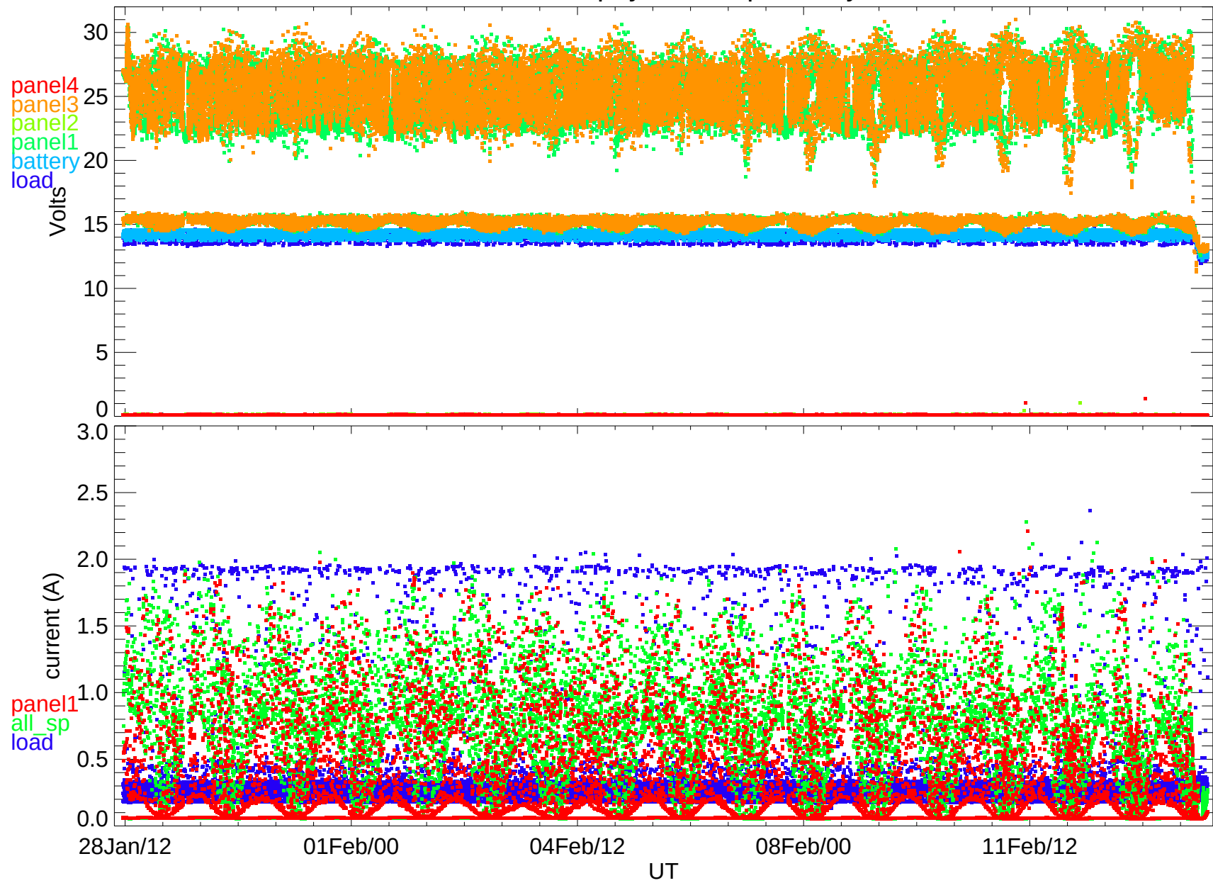
BARREL 2013 payload 1A power system
