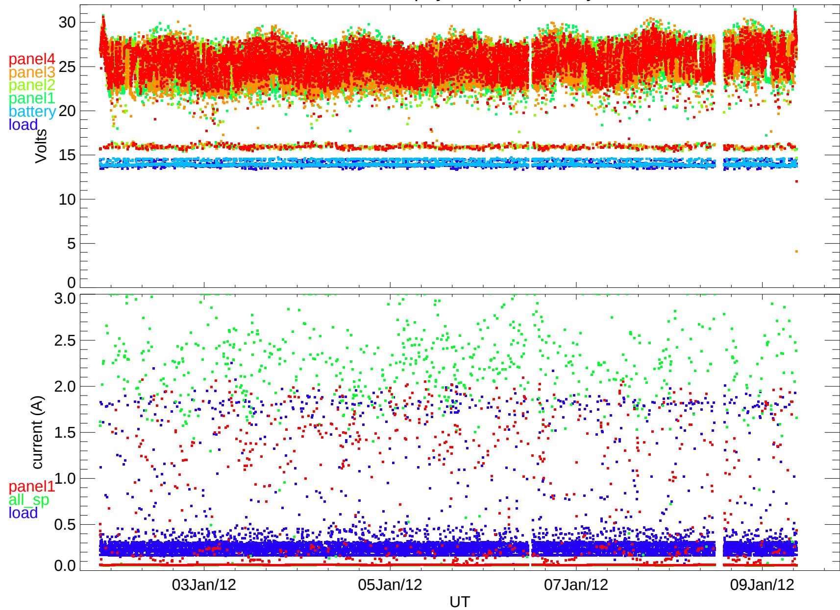
BARREL 2013 payload 1B power system
