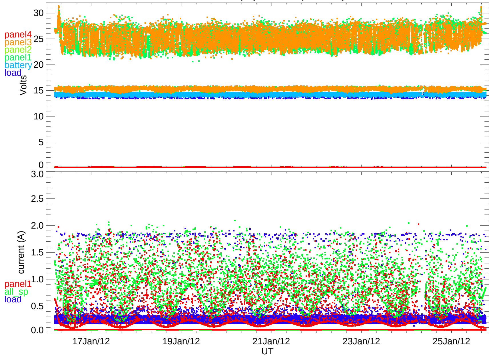
BARREL 2013 payload 1C power system
