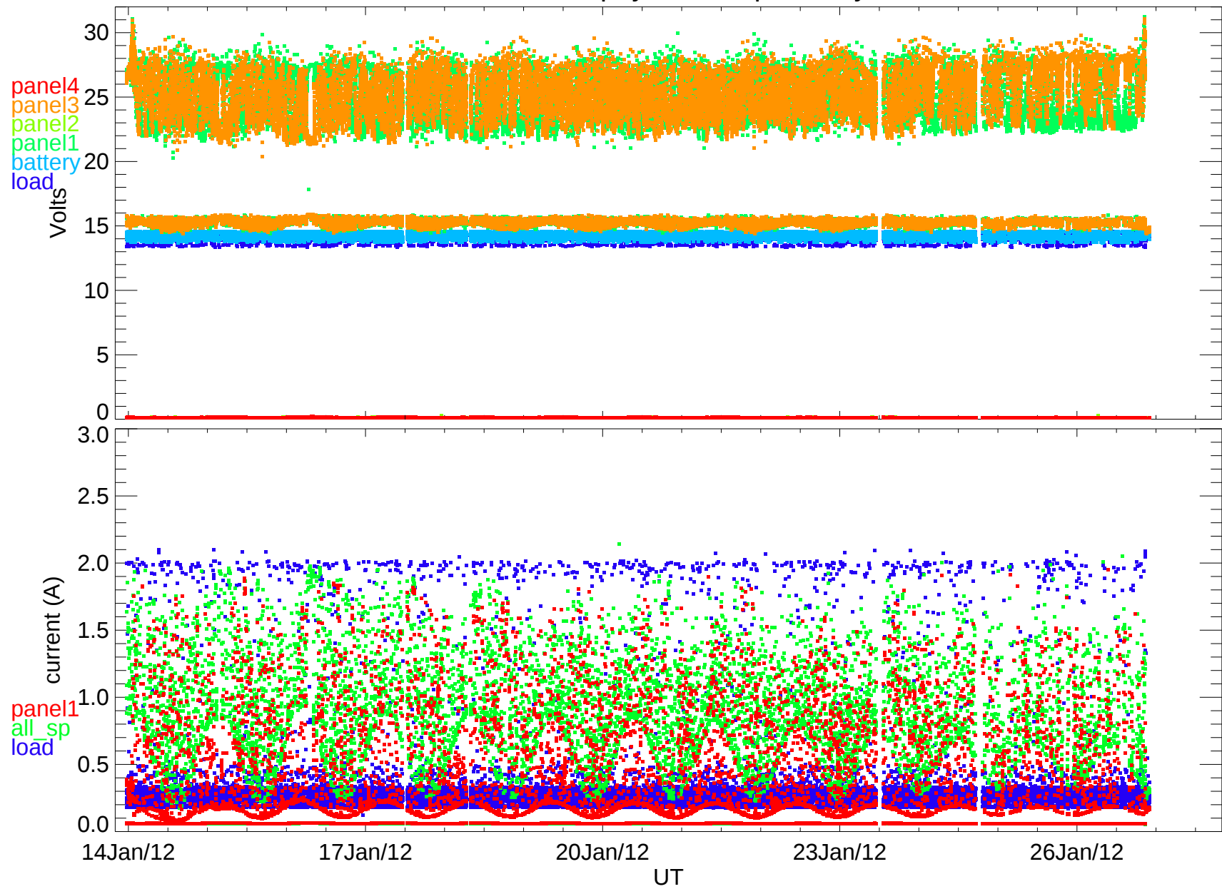
BARREL 2013 payload 1G power system
