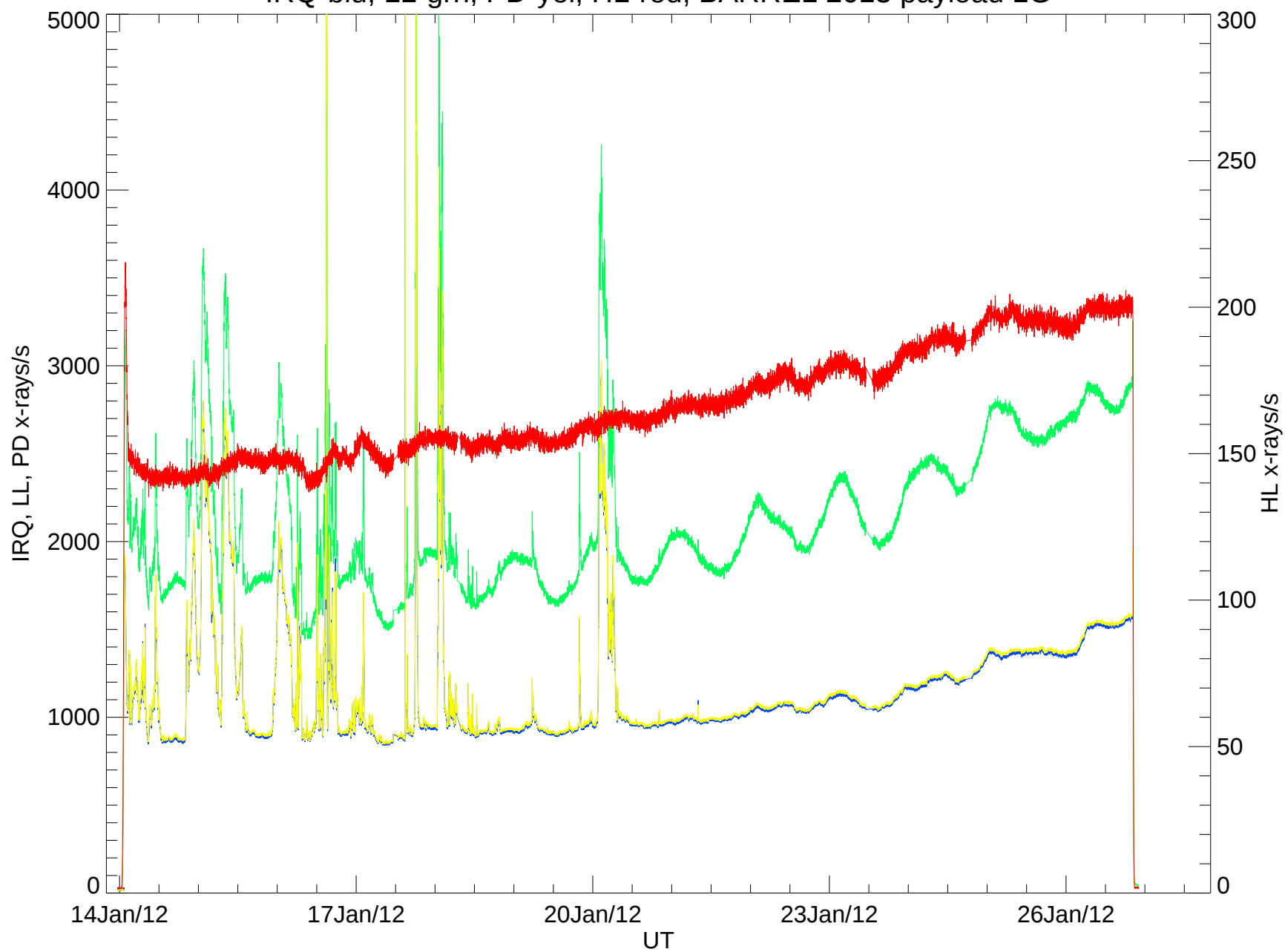
IRQ-blu, LL-grn, PD-yel, HL-red; BARREL 2013 payload 1G
