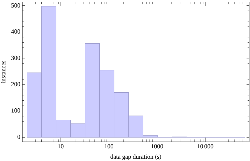
BARREL 2013 payload 1H 0.0632 dropped
