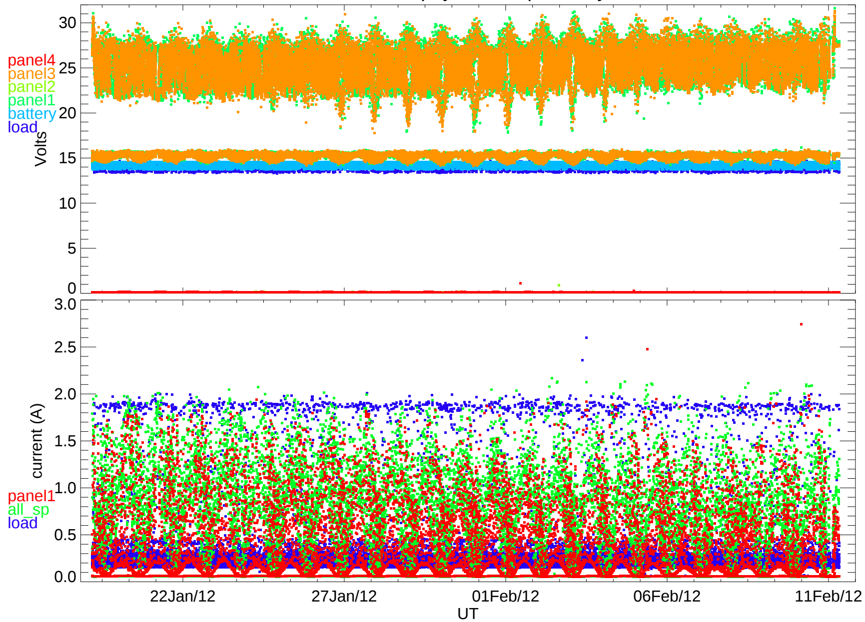
BARREL 2013 payload 1H power system
