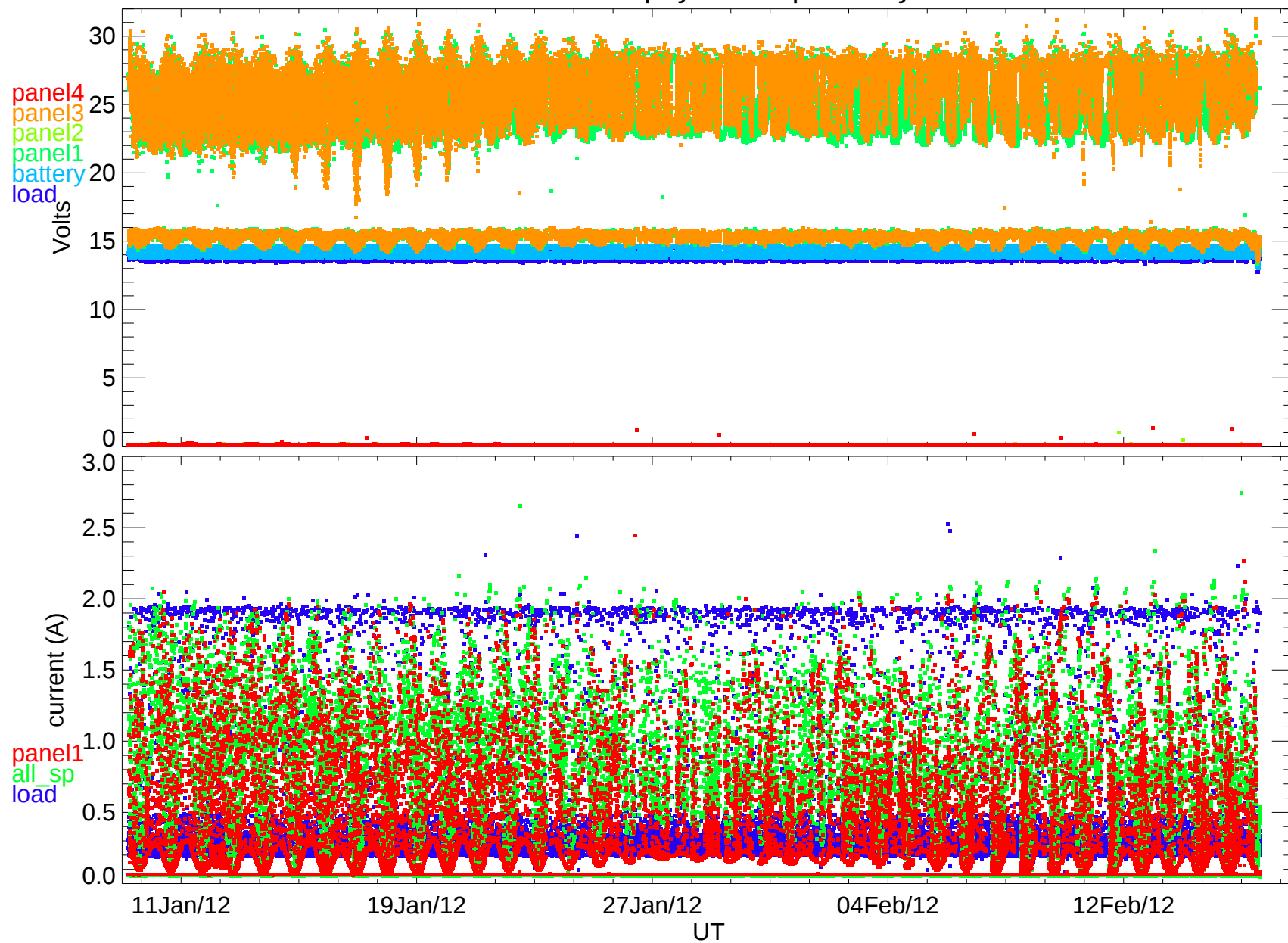
BARREL 2013 payload 1I power system
