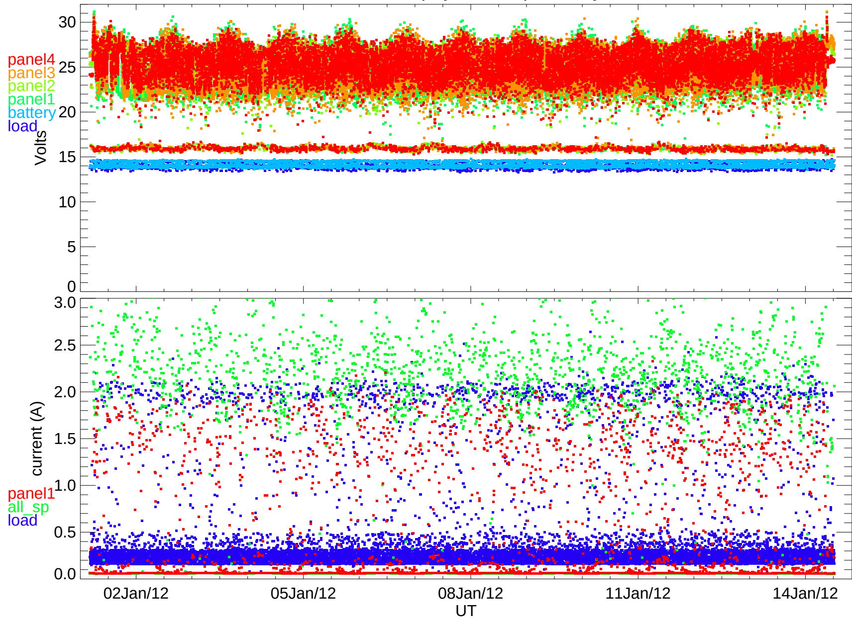
BARREL 2013 payload 1J power system
