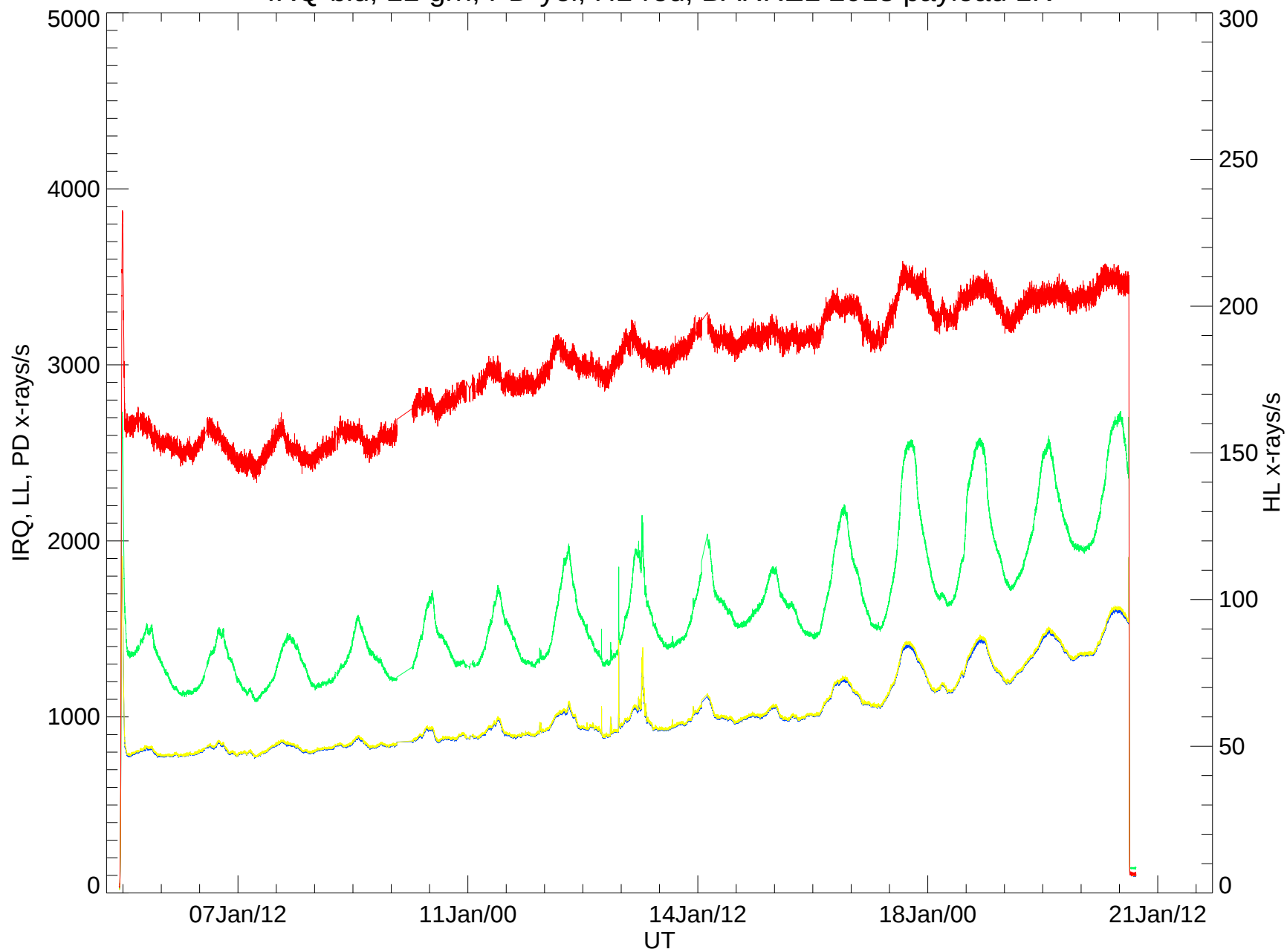
IRQ-blu, LL-grn, PD-yel, HL-red; BARREL 2013 payload 1K
