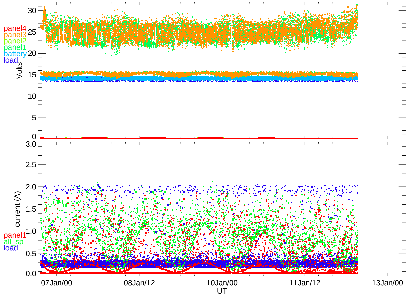
BARREL 2013 payload 1M power system
