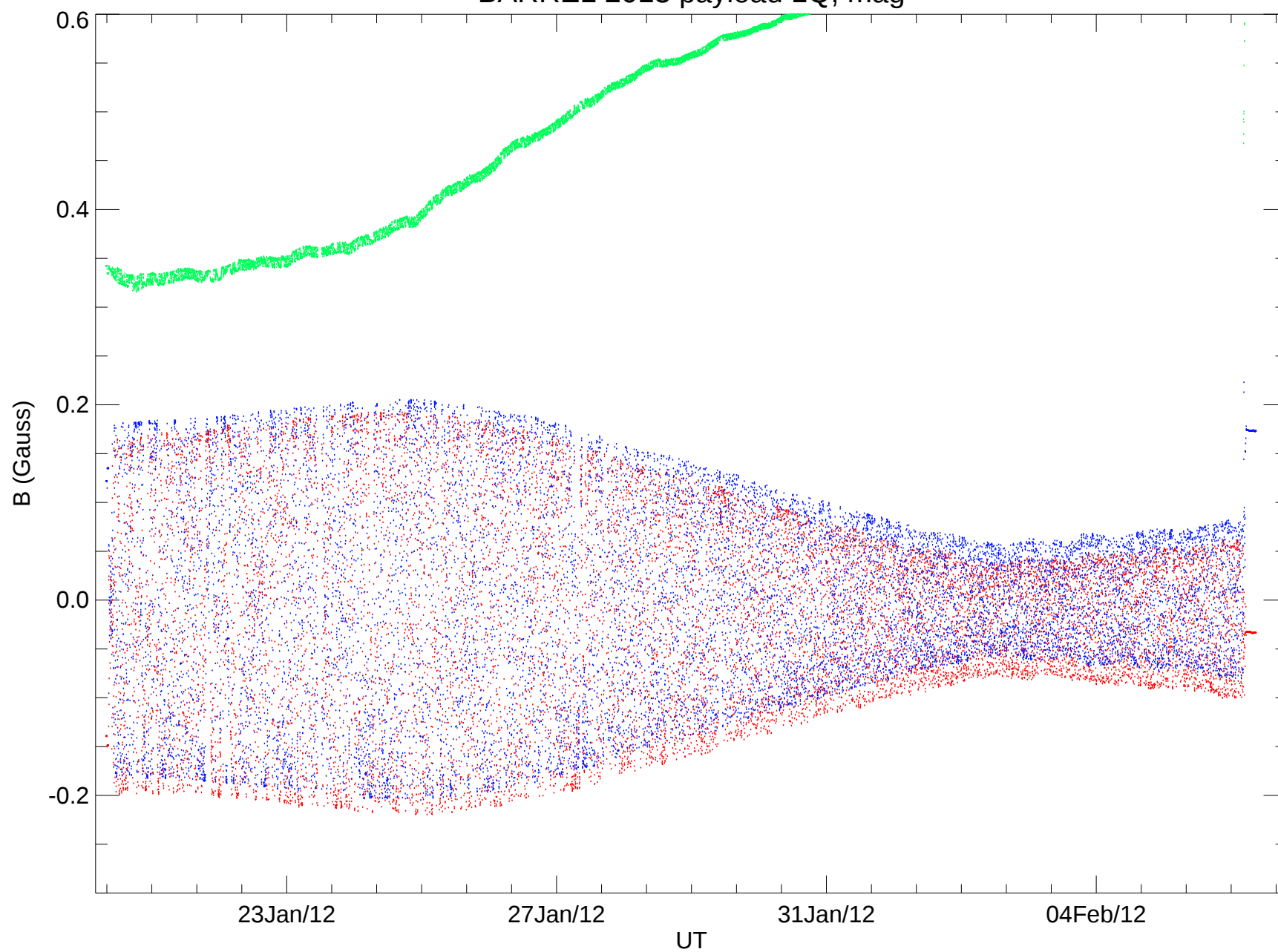
BARREL 2013 payload 1Q; mag
