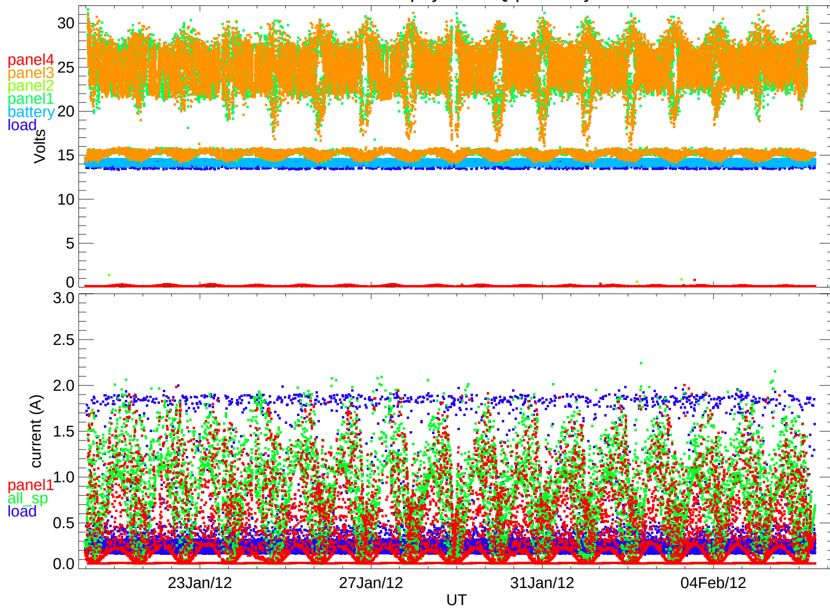
BARREL 2013 payload 1Q power system
