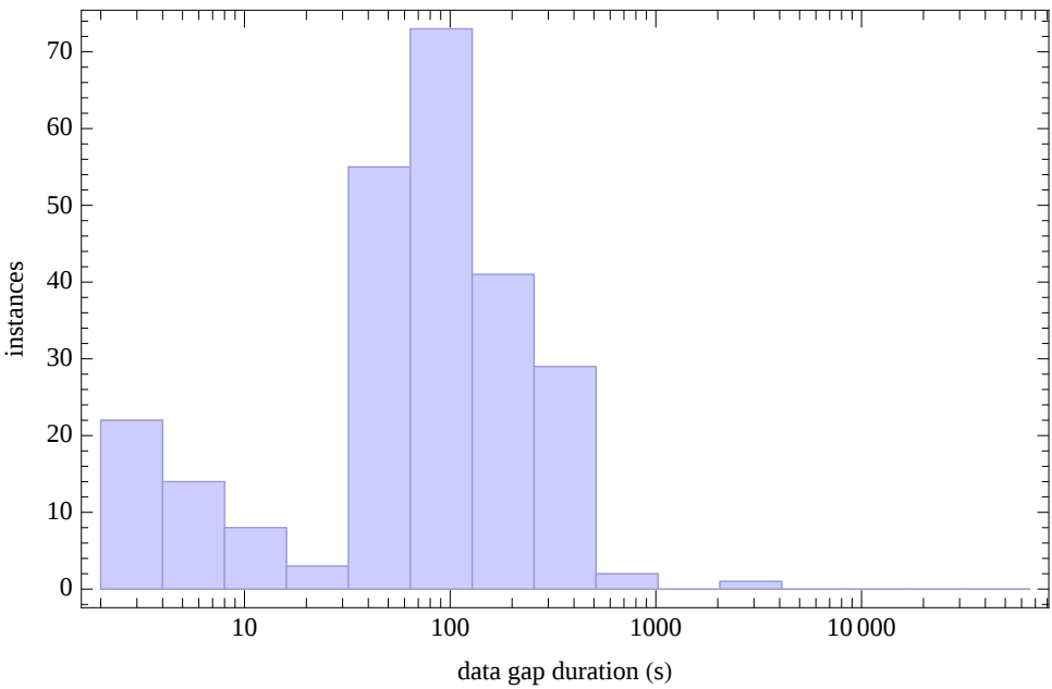
BARREL 2013 payload 1S 0.0790 dropped
