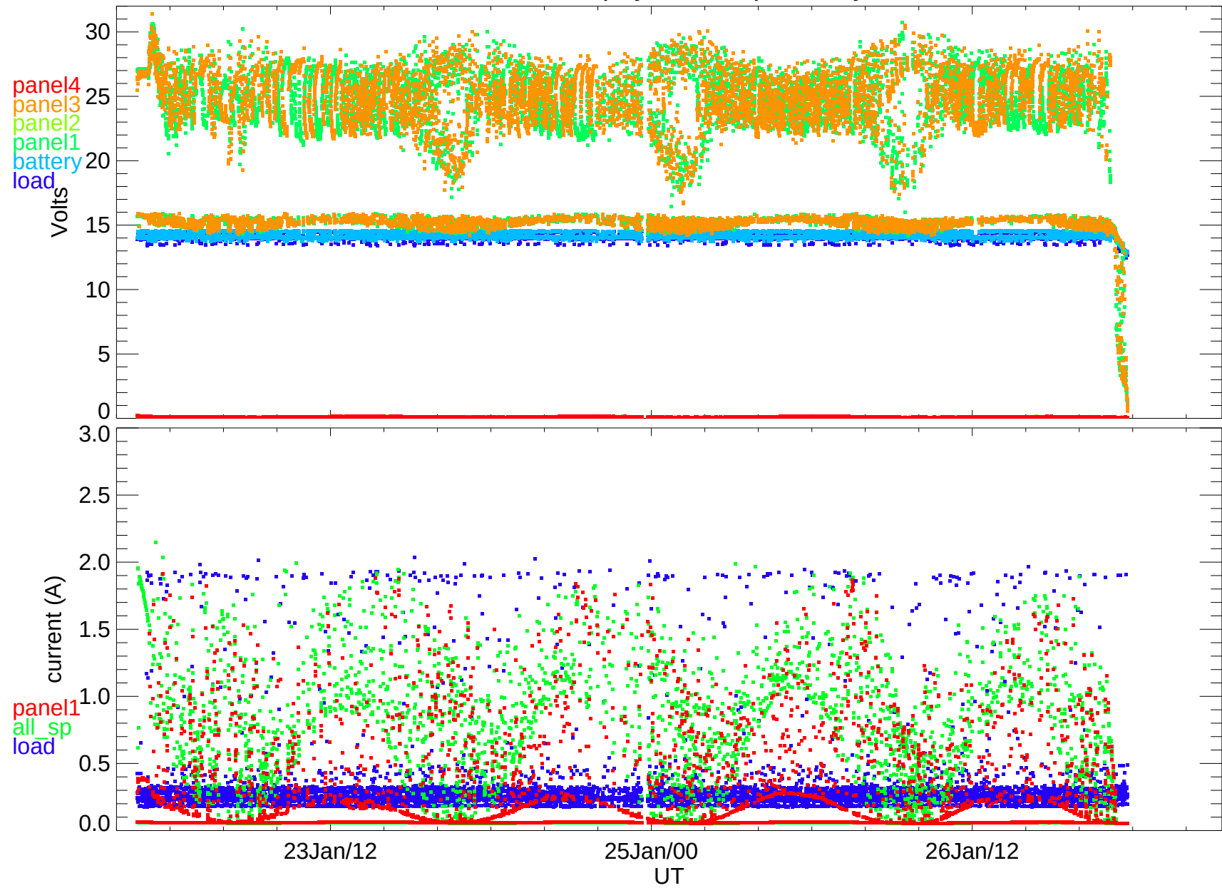
BARREL 2013 payload 1S power system
