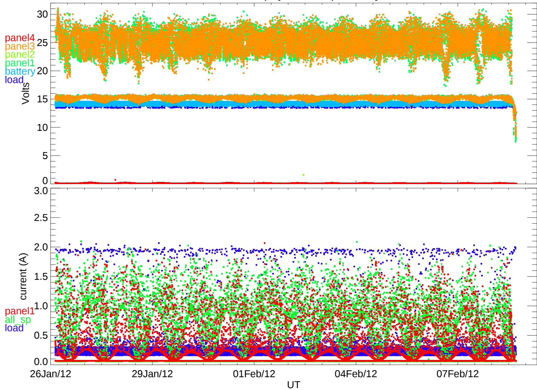
BARREL 2013 payload 1U power system
