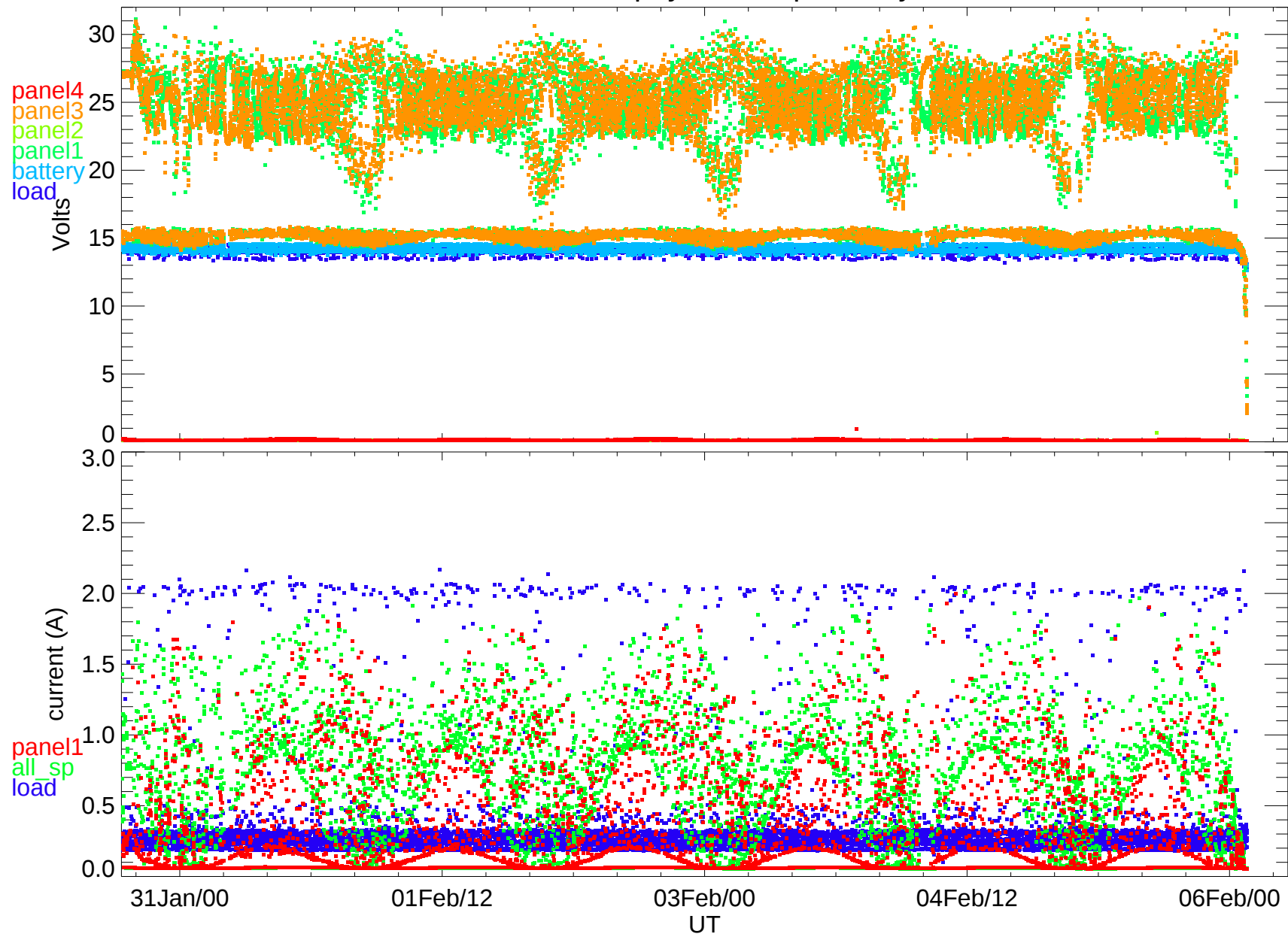
BARREL 2013 payload 1V power system
