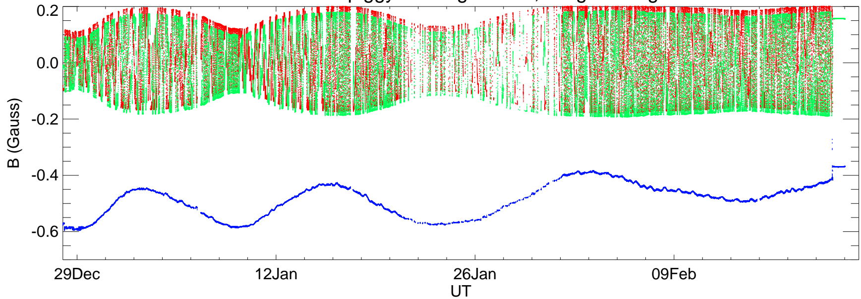
BARREL piggyback flight 2008; fluxgate mag
