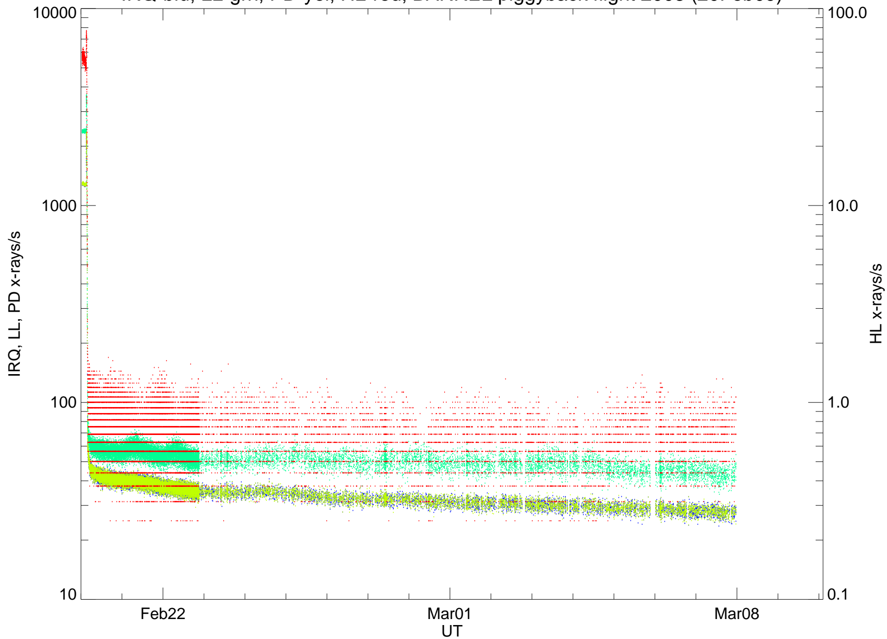
IRQ-blu, LL-grn, PD-yel, HL-red; BARREL piggyback flight 2008 (20Feb09)
