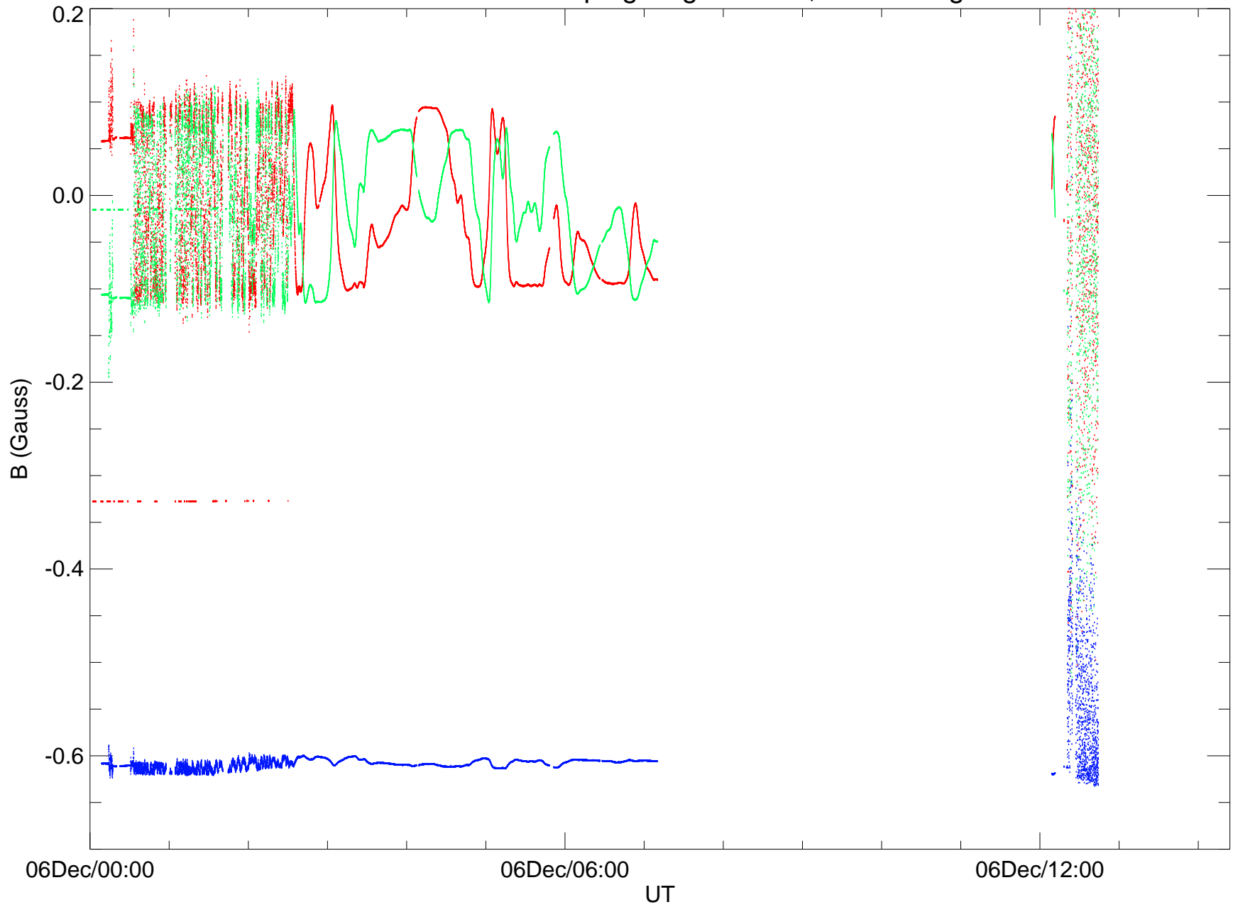
BARREL test campaign flight2 2009; TCM3 mag
