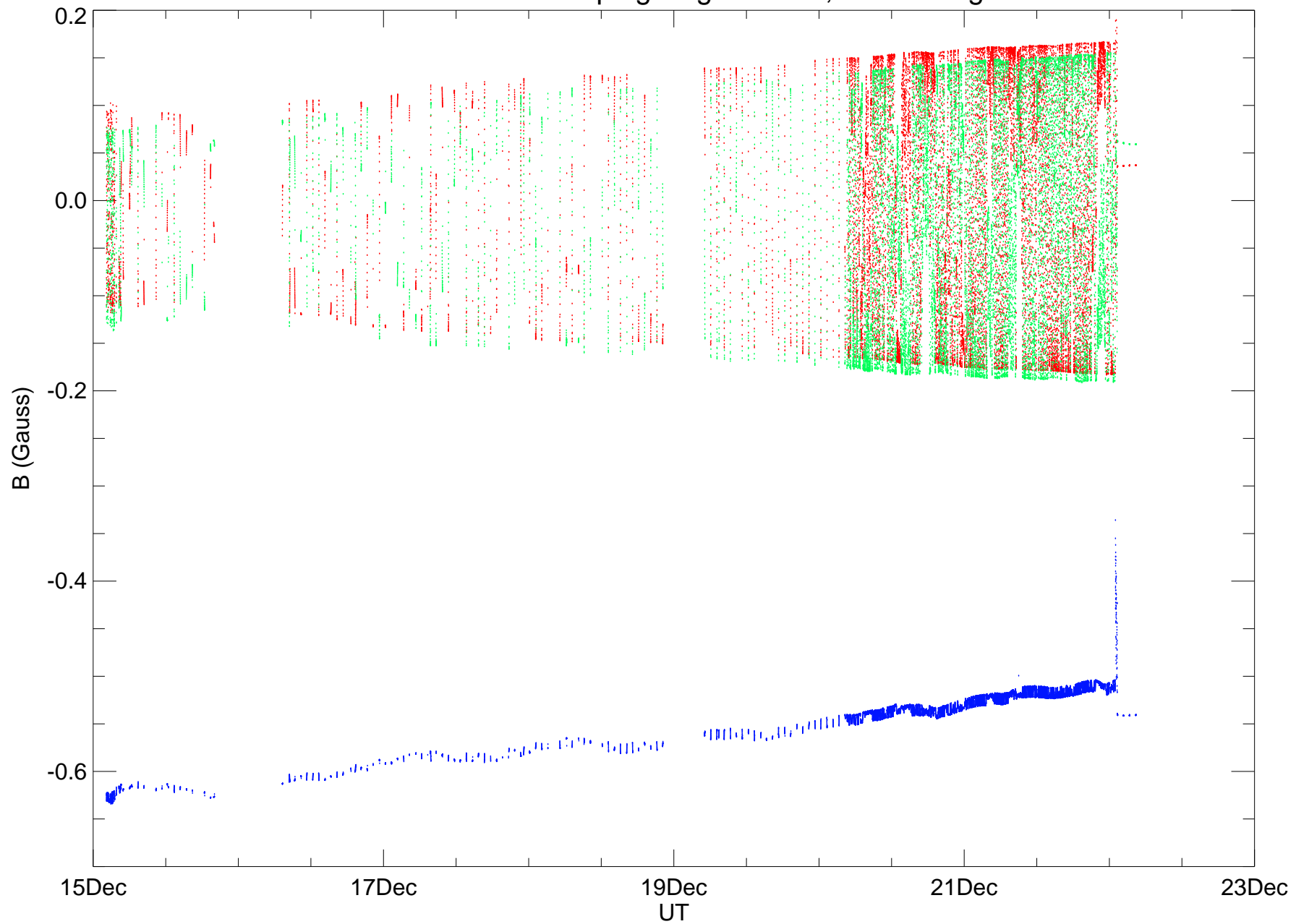
BARREL test campaign flight3 2009; TCM3 mag
