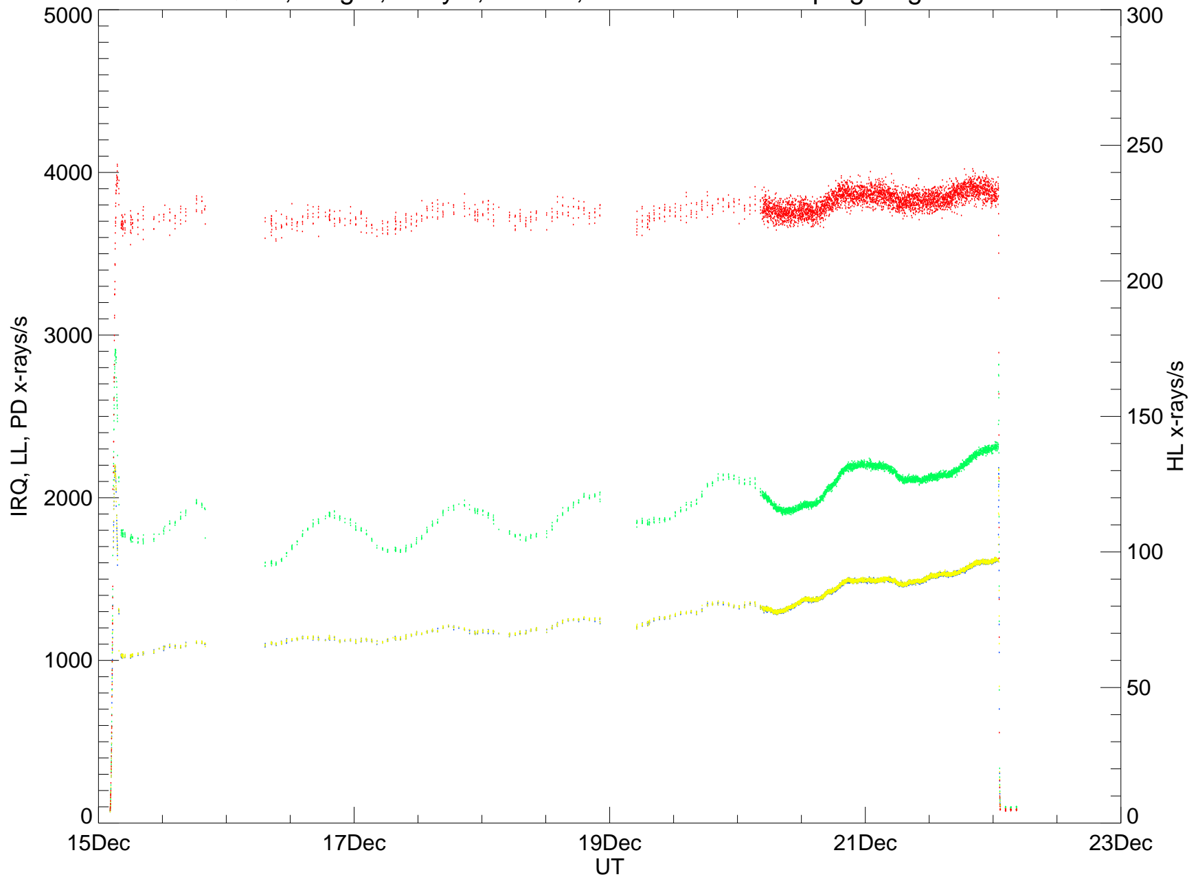
IRQ-blu, LL-grn, PD-yel, HL-red; BARREL test campaign flight3 2009
