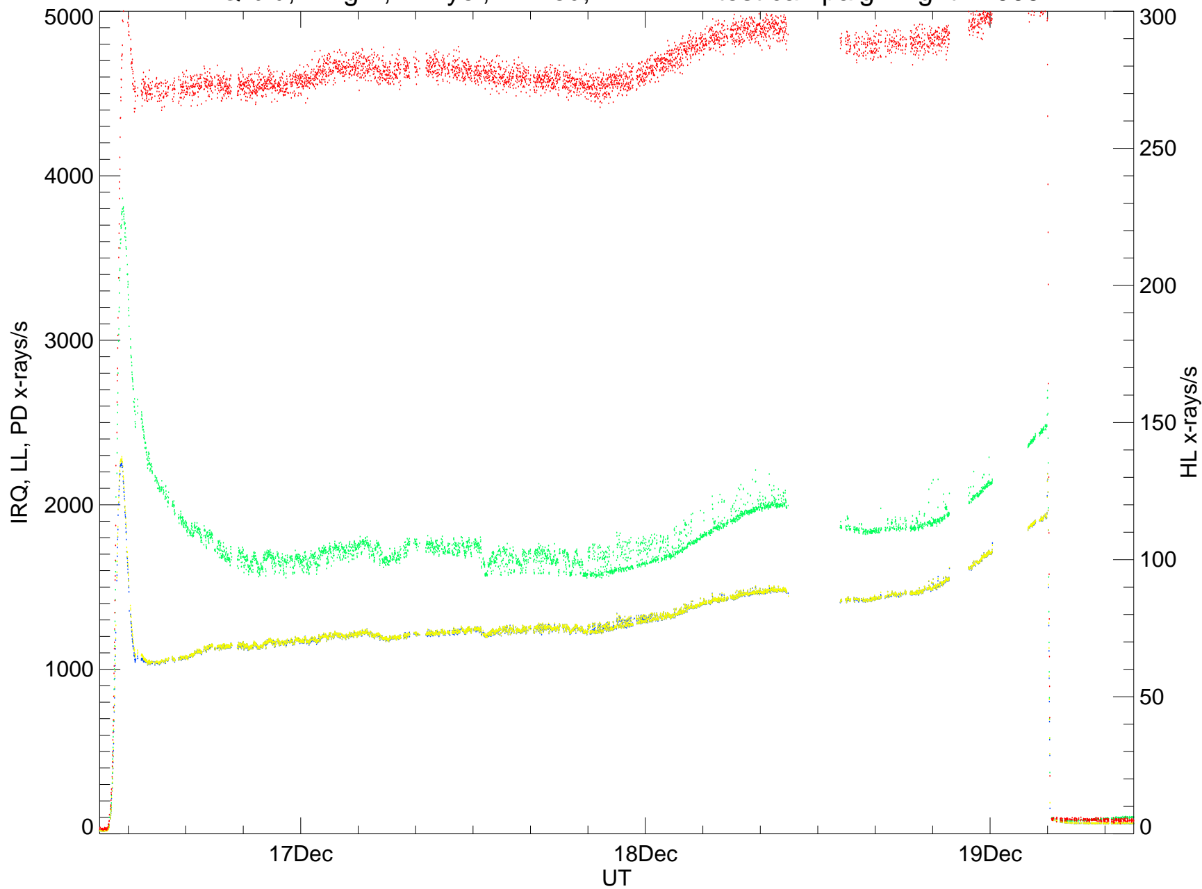
IRQ-blu, LL-grn, PD-yel, HL-red; BARREL test campaign flight4 2009
