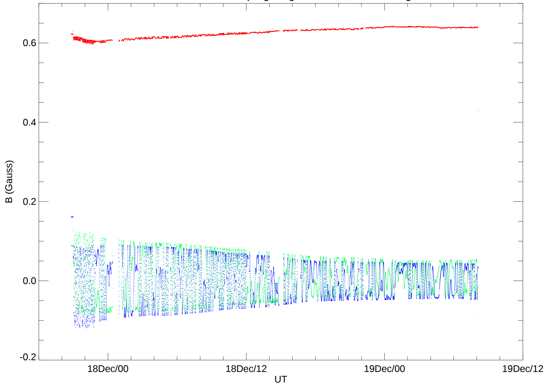
BARREL test campaign flight 6 2010; TCM3 mag
