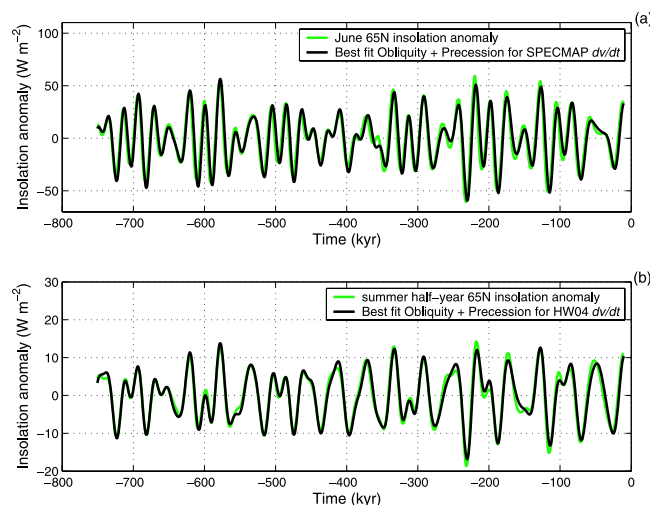
Figure 3. Results of optimized linear regression of climatic precession and obliquity indices onto the rate of change of ice volume allowing for arbitrary amplitude and lag, compared to indices of summer insolation variations at 65N, using (a) the SPECMAP record and (b) the HW04 record. The results of the linear regression are scaled to the insolation index in Figures 3a and 3b. Note the different scales on the y-axes. See auxiliary materials for methods.
